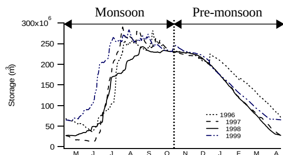
Fig.2 Storage Curve of Reservoir (1996~1999)
